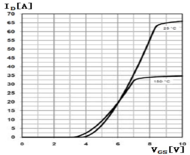
Transfer Characteristic
